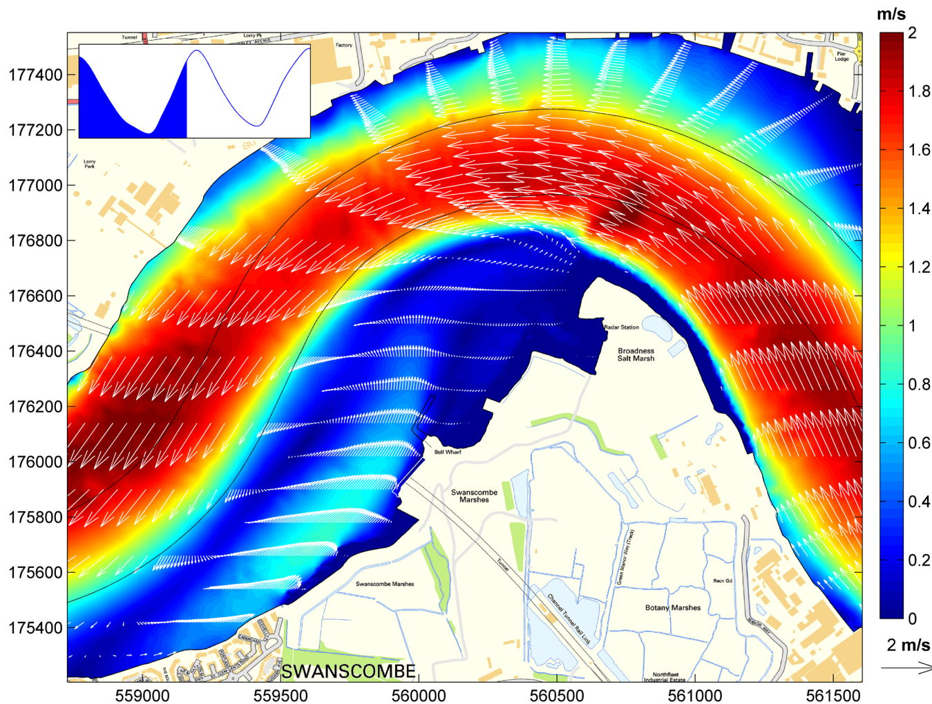
Figure 17.19: Kent Project Site Baseline Hydrodynamic showing current magnitude at time peak flood tide.
